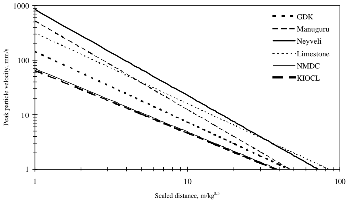
Fig. 2.8 Comparison of peak particle velocities for different surface mines
