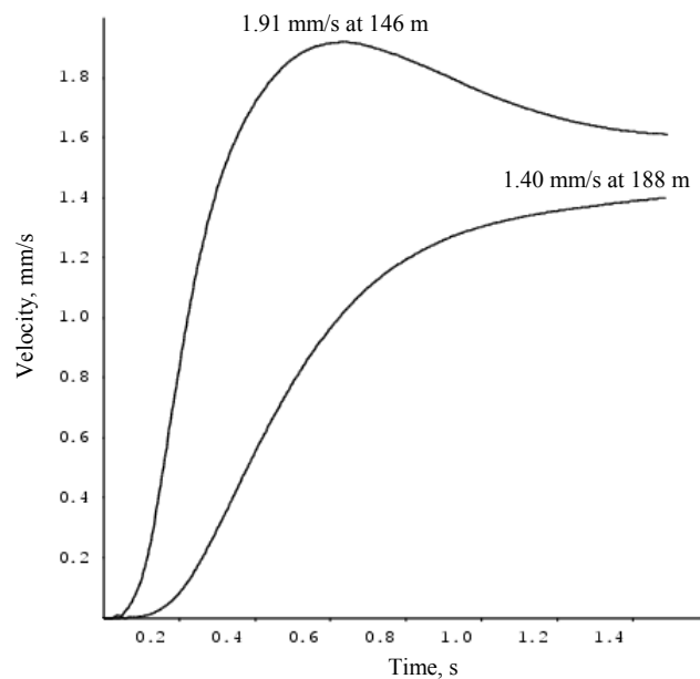
Fig. 8.8 Generated vibration histories at two locations with a trench equal to hole depth
