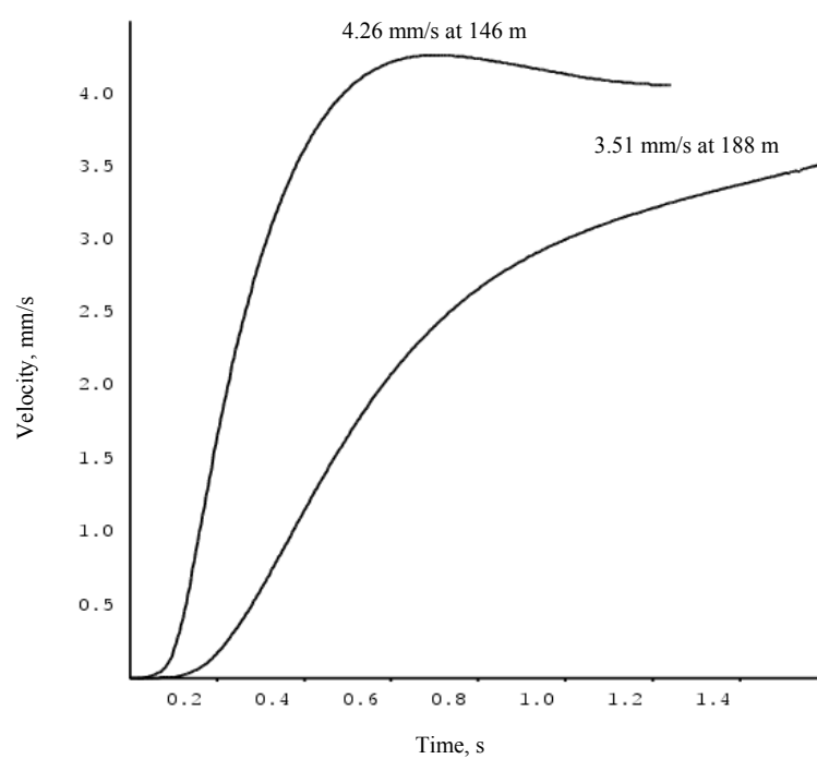
Fig. 8.5 Generated vibration histories - calibrated model
