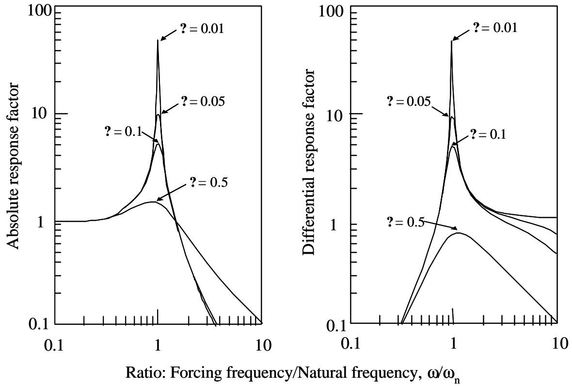
Fig. 5.2 Simulation of structure response using a single degree of freedom model (Crum and Pierce, 1995)
