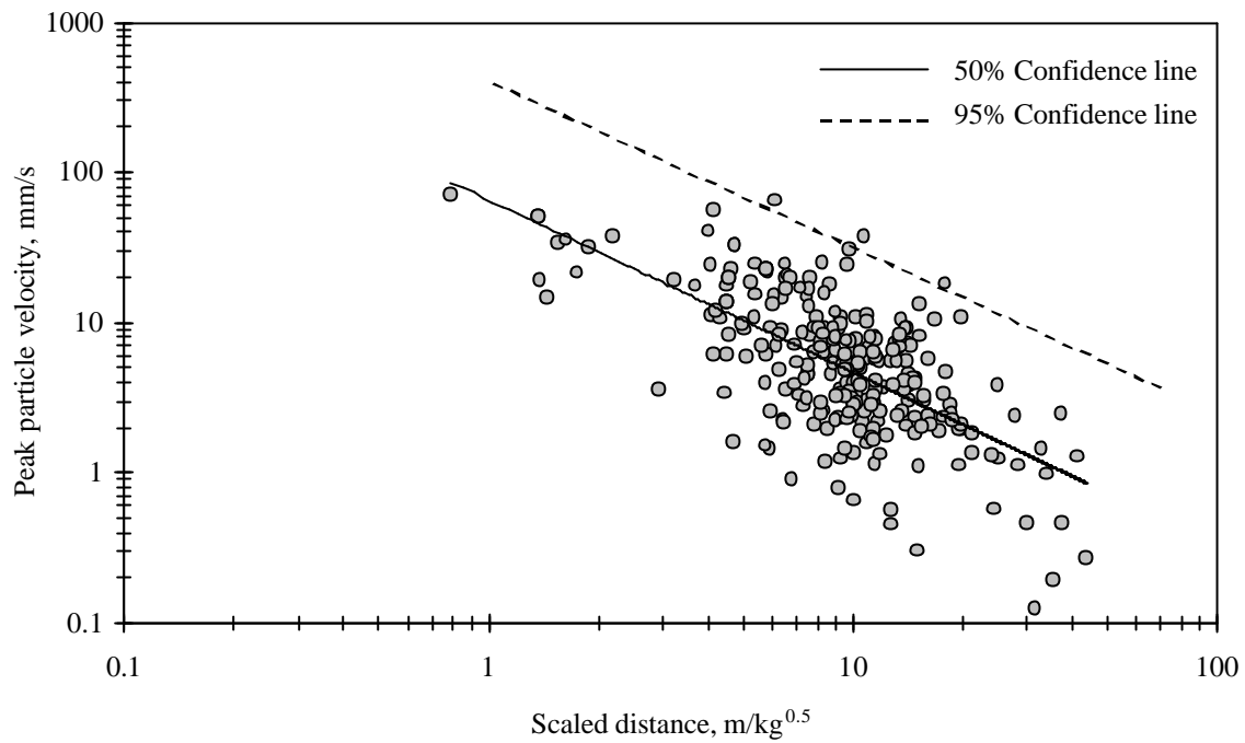
Fig. 2.5 Peak particle velocity vs scaled distance for Kudremukh iron ore mine
