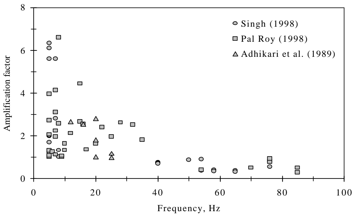
Fig. 5.3 Previous work on amplification factor in India
