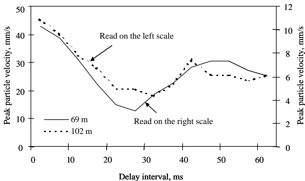
Fig. 7.10 Influence of delay interval on peak particle velocity at OC-2, SCCL
