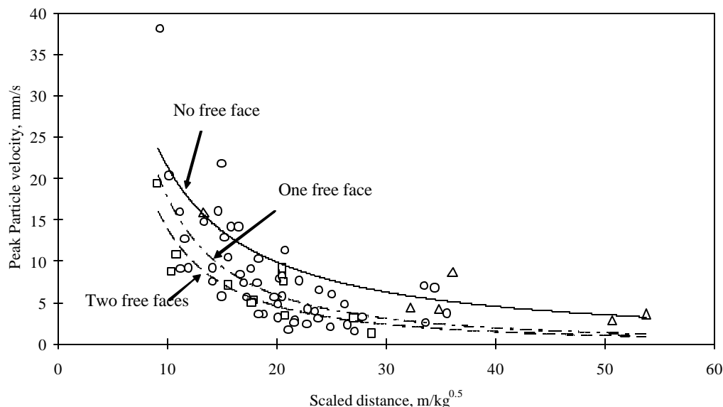
Fig. 7.6 Influence of free faces on peak particle velocity at Kamptee OCP, WCL
