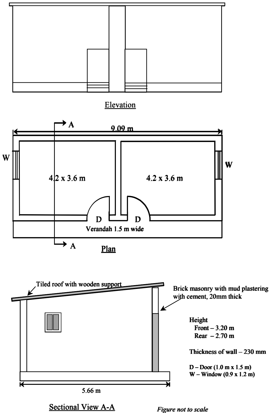
Fig. 3.7 Plan and section of the single storey structure at OC-2, SCCL
