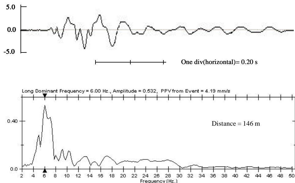
Fig. 7.3 Single hole waveform and its frequency analysis for Kamptee OCP, WCL
