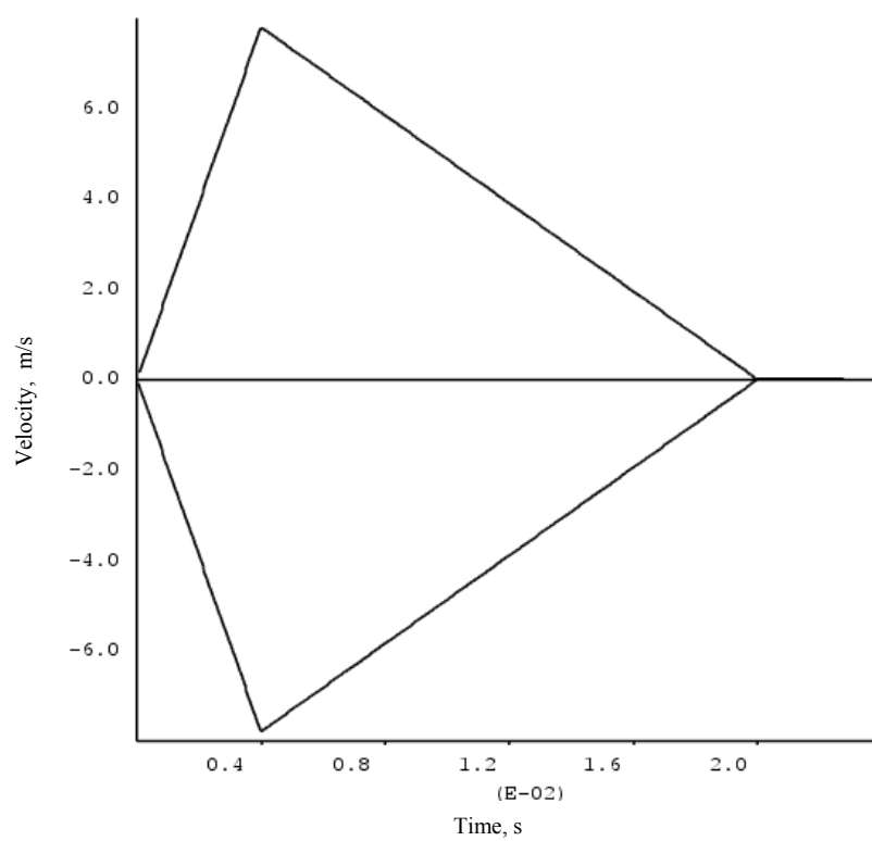
Fig. 8.4 Loading of blasthole with a triangular pulse – 7.8 m/s velocity
