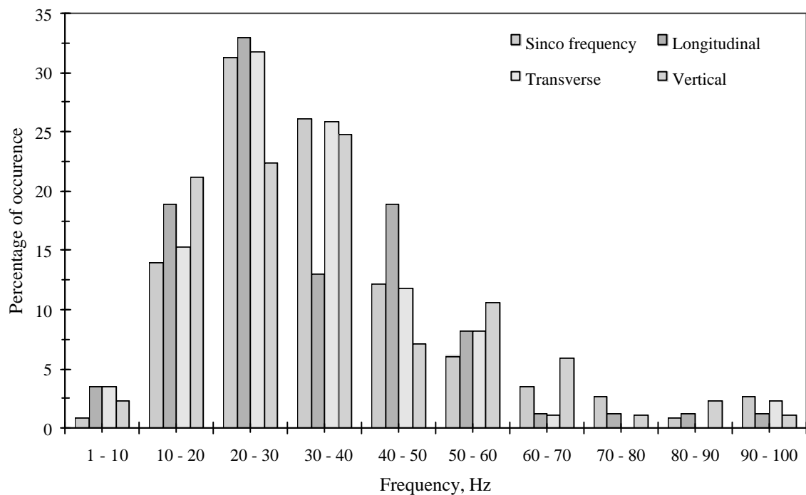
Fig. 2.12 Frequency content of ground vibration for limestone mines (Adhikari et al, 2004)
