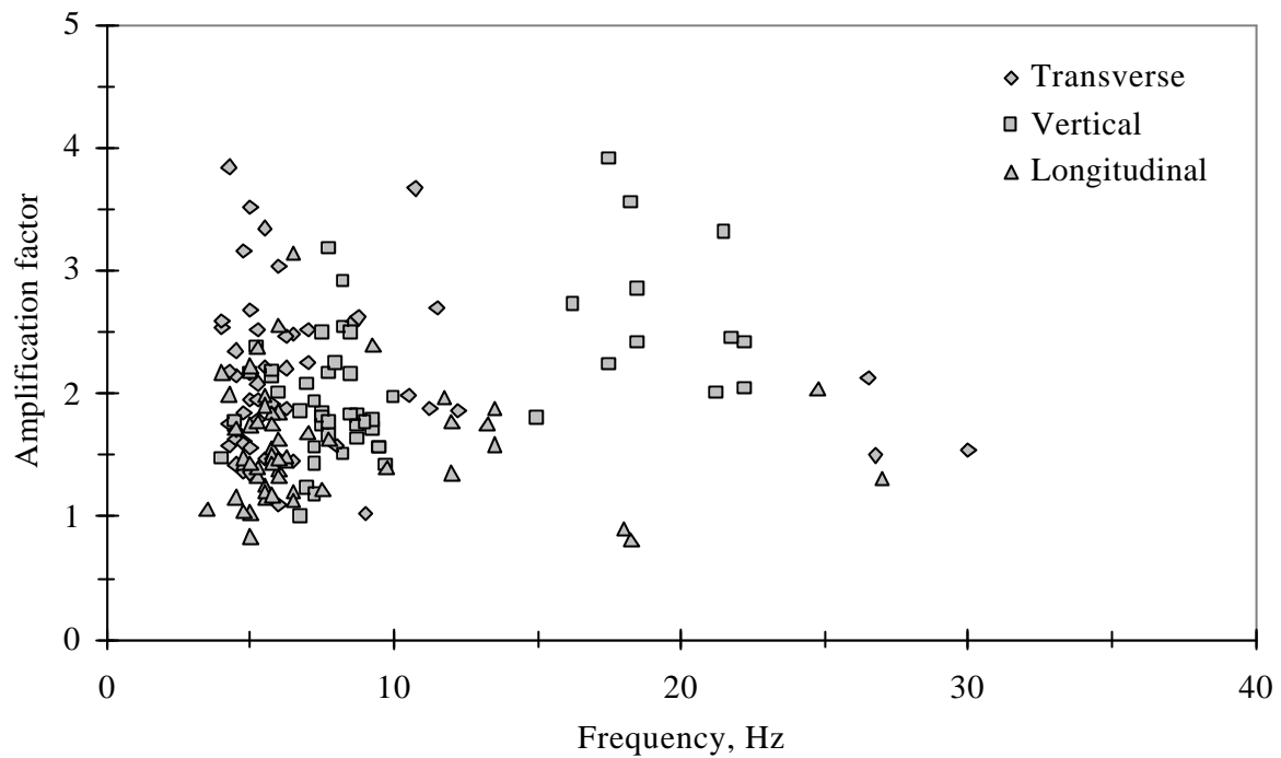
Fig. 5.5 Amplification factor versus frequency of ground vibration at Kamptee OCP, WCL
