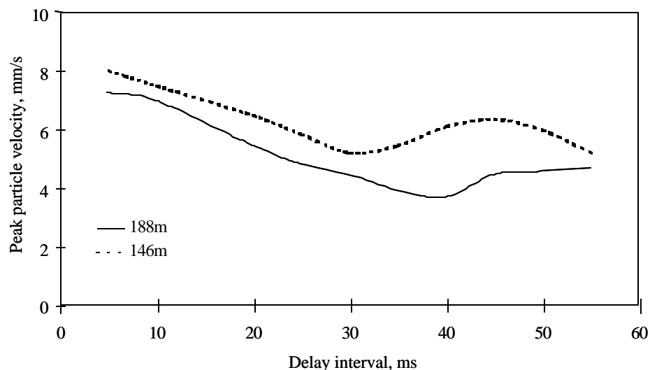
Fig. 7.4 Influence of delay interval on peak particle velocity at Kamptee OCP, WCL
