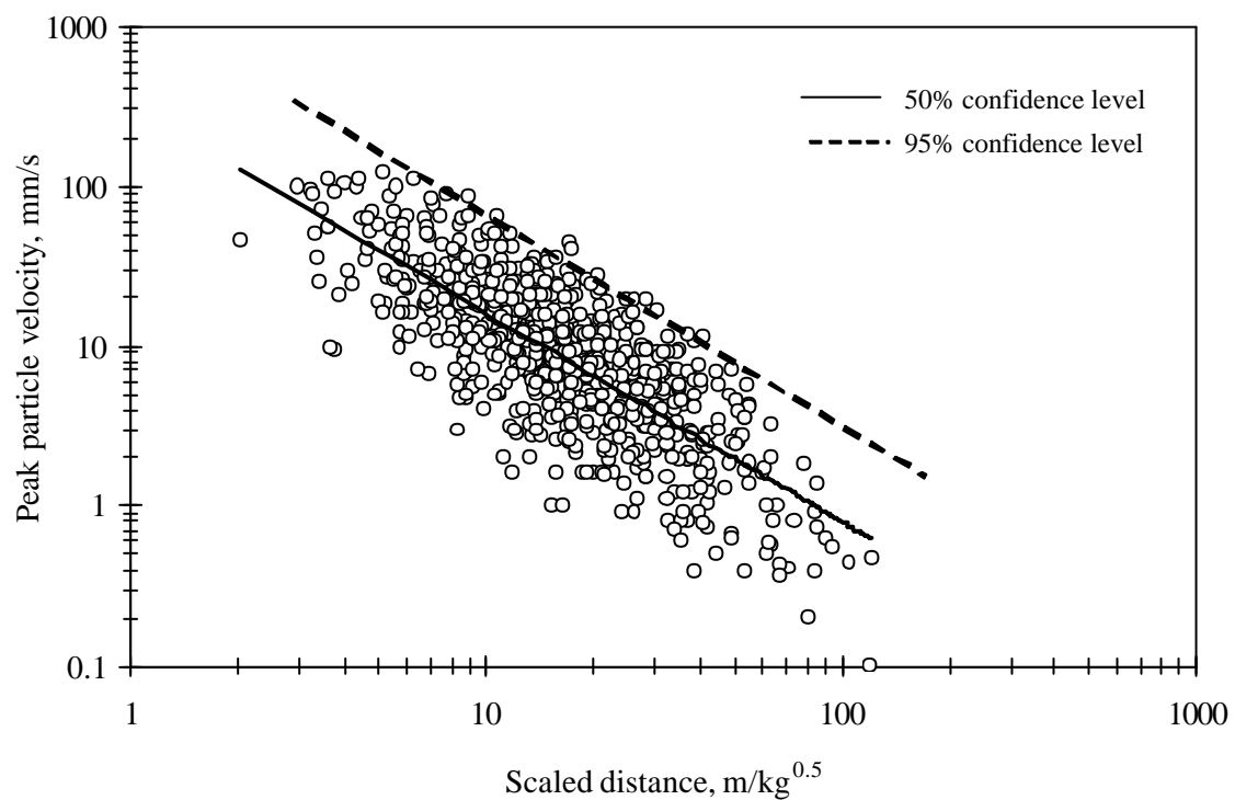
Fig. 2.6 Peak particle velocity vs scaled distance for limestone quarries (Adhikari et al, 2004)
