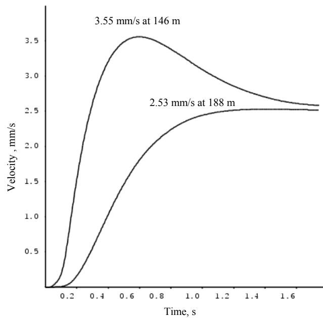
Fig. 8.7 Generated vibration histories at two locations with a trench equal to half the hole depth
