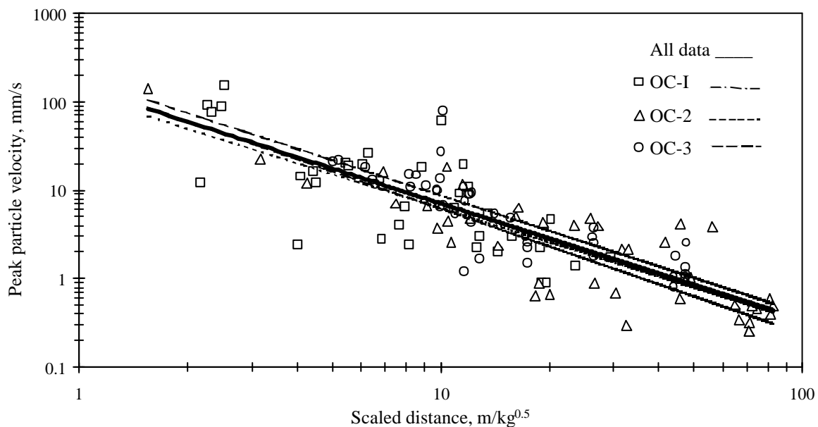
Fig. 2.1 Peak particle velocity vs scaled distance for Godavarikhani area (Theresraj et al, 2003)
