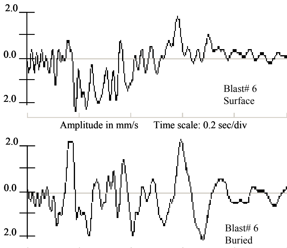
Fig. 4.10 Distorted waveform of the surface transducer compared to the undistorted one of the buried transducer (Blast # 6)
