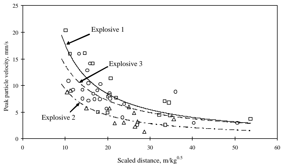
Fig. 7.5 Influence of explosives on ground vibration at Kamptee OCP, WCL
