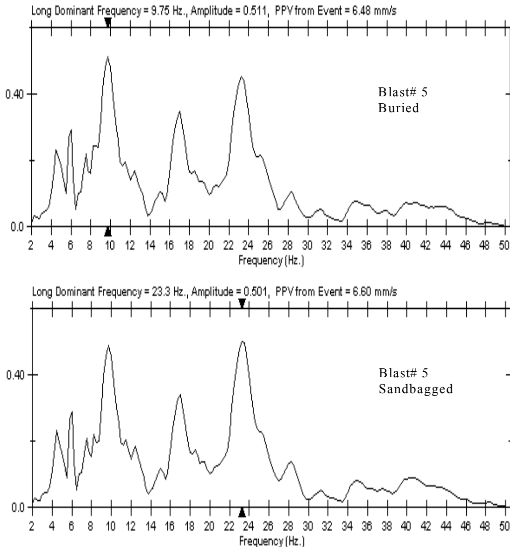
Fig. 4.5 Comparison of frequency spectra - buried and sandbagged transducers (Blast #5).
