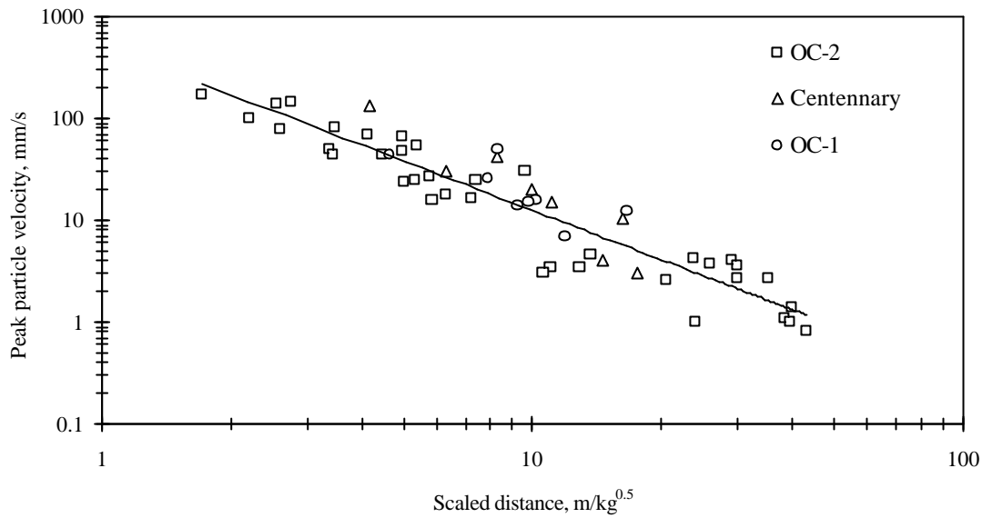
Fig. 2.2 Peak particle velocity vs scaled distance for Manuguru area, SCCL
