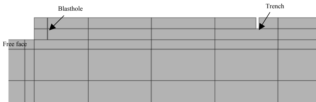
Fig. 8.6 Creation of a trench with its depth equal to half the hole depth
