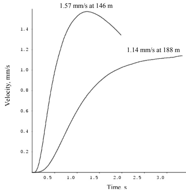
Fig. 8.9 Generated vibration histories at two locations with a trench equal to one and half times the hole depth
