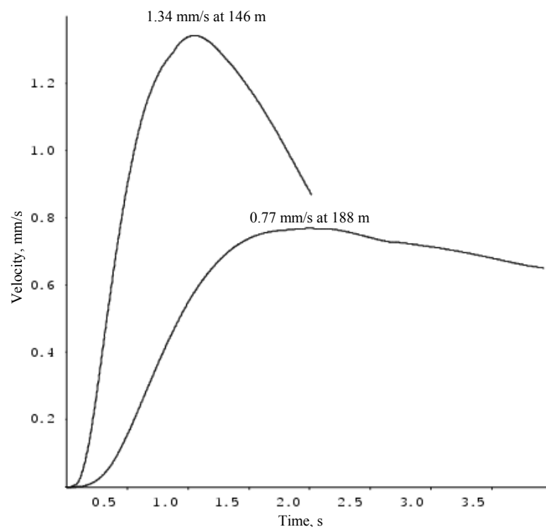
Fig. 8.10 Generated vibration histories at two locations with a trench equal to twice the hole depth
