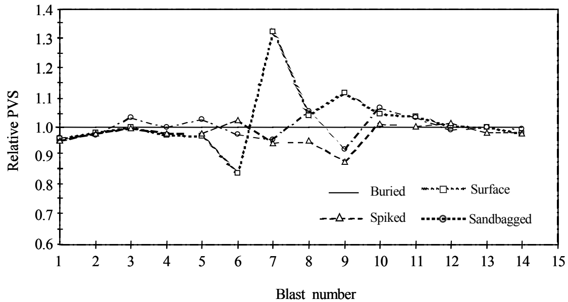
Fig. 4.2 Influence of the transducer mounting methods on peak particle velocity (PPV)
