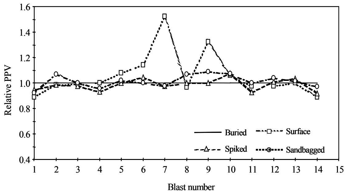
Fig. 4.3 Influence of the transducer mounting methods on peak vector sum (PVS)
