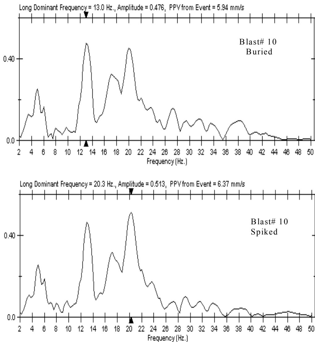
Fig. 4.7 Comparison of frequency spectra - buried and spiked transducers (Blast #10).
