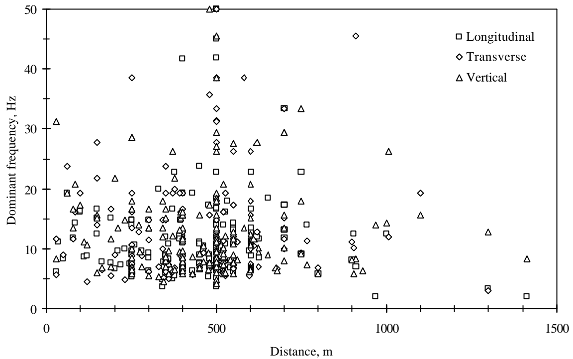
Fig. 2.11 Dominant frequency vs distance for Kudremukh iron ore mine
