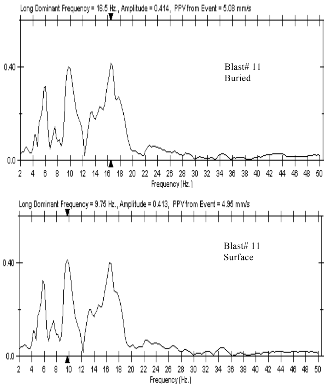
Fig. 4.6 Comparison of frequency spectra - buried and surface transducers (Blast #11).
