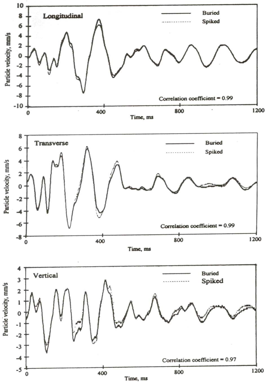
Fig. 4.9 Superimposed waveforms of the buried and spiked transducers (Blast # 2)
