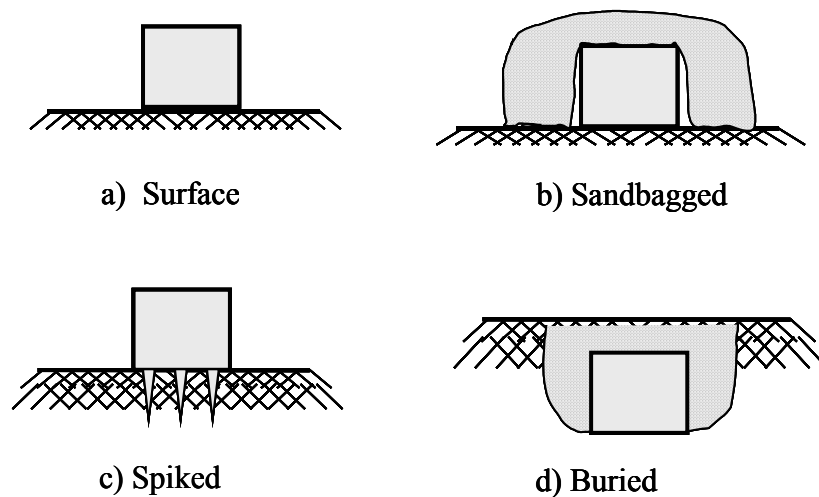
Fig. 4.1 Four common methods of transducer mounting
