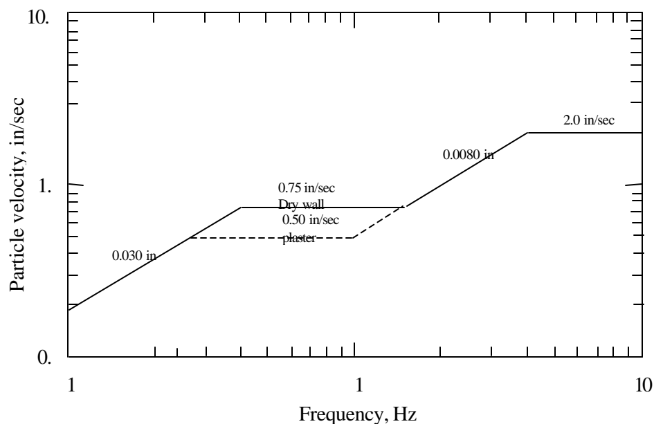
Fig. A Safe limits of blast vibration for houses (Siskind et al, 1980)
