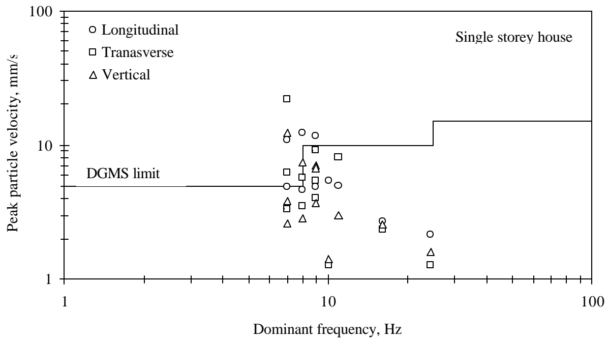
Fig. 6.2 Measured ground vibrations vis-a-vis DGMS limits for second structure at Kamptee OCP
