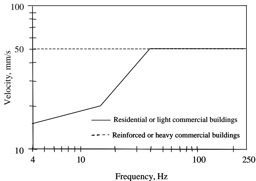
Fig. B British Standard BS 7385 of 1993
