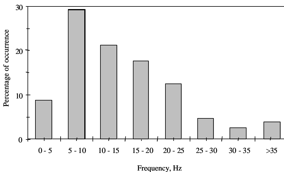
Fig. 7.9 Frequency of ground vibration at OC-2, SCCL
