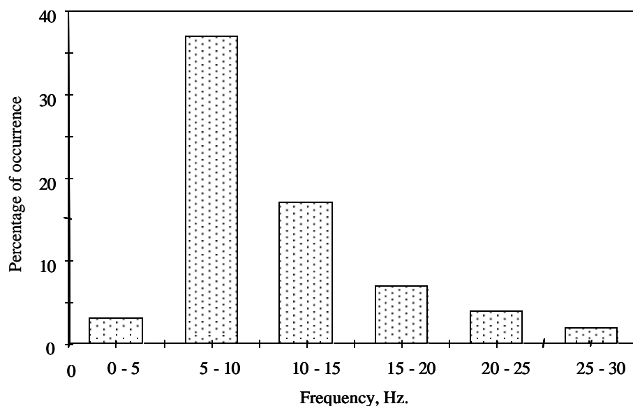
Fig. 7.2 Frequency of ground vibration at Kamptee OCP
