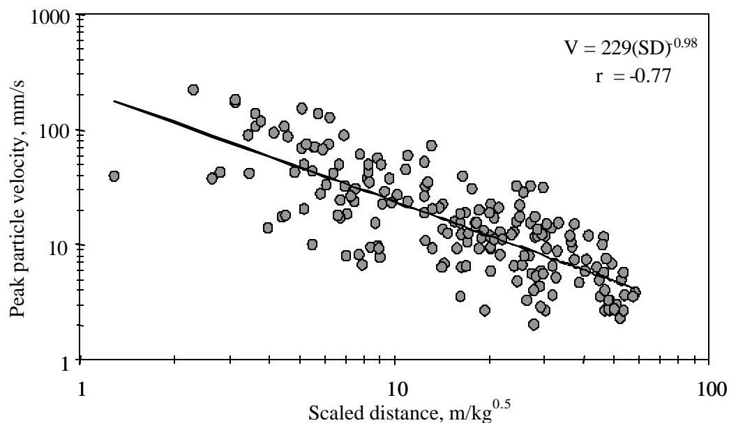
Fig. 7.8 Peak particle velocity versus scaled distance for OC-2, SCCL
