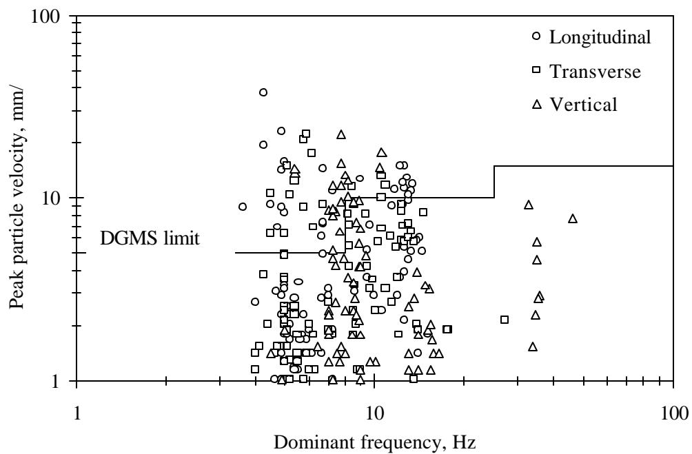
Fig. 6.6 Measured ground vibrations vis-a-vis the DGMS limits for double storey structure at OC-2
