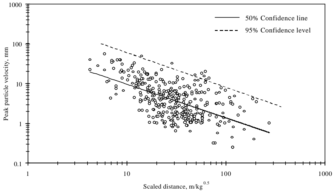
Fig. 2.7 Peak particle velocity vs scaled distance for construction projects (Adhikari et al, 2005)
