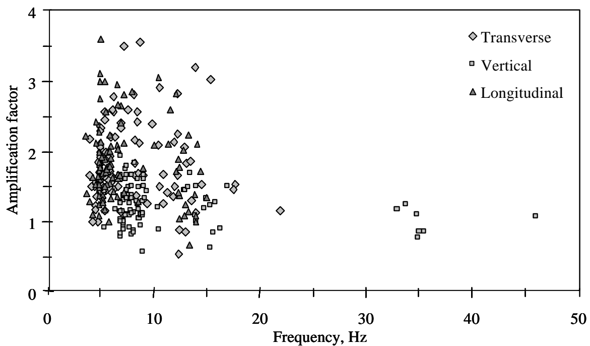
Fig. 5.6 Amplification factor versus frequency of ground vibration at OC-2, SCCL
