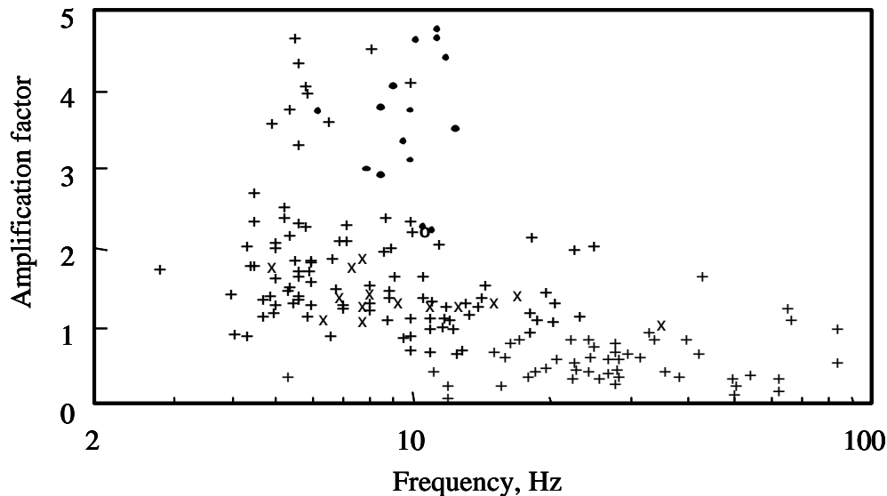
Fig. 5.1 Amplification factor versus frequency of ground vibration (Siskind, 2000)
