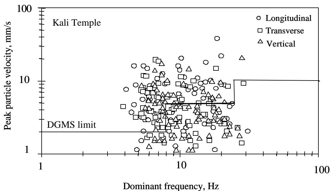
Fig. 6.4 Measured ground vibrations vis-a-vis DGMS limits for fourth structure at Kamptee OCP
