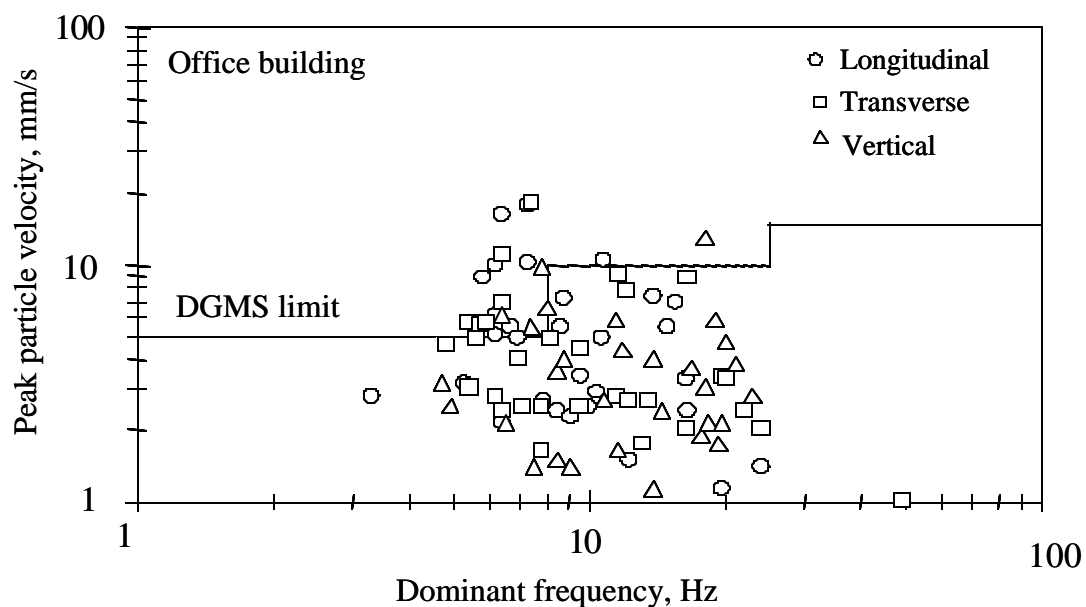
Fig. 6.3 Measured ground vibrations vis-a-vis DGMS limits for third structure at Kamptee OCP
