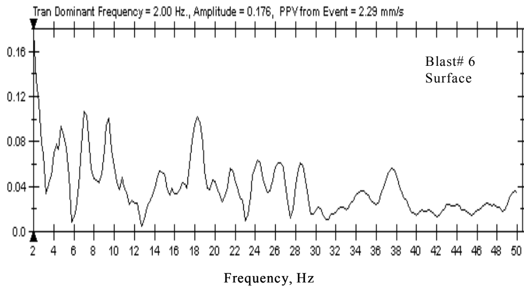
Fig. 4.8 Frequency spectra showing the presence of a very low frequency (Blast #6)
