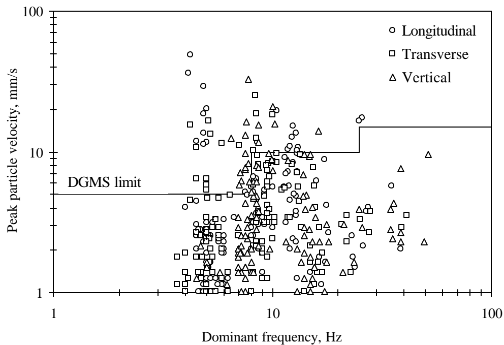
Fig. 6.5 Measured ground vibrations vis-a-vis the DGMS limits for single storey structure at OC-2
