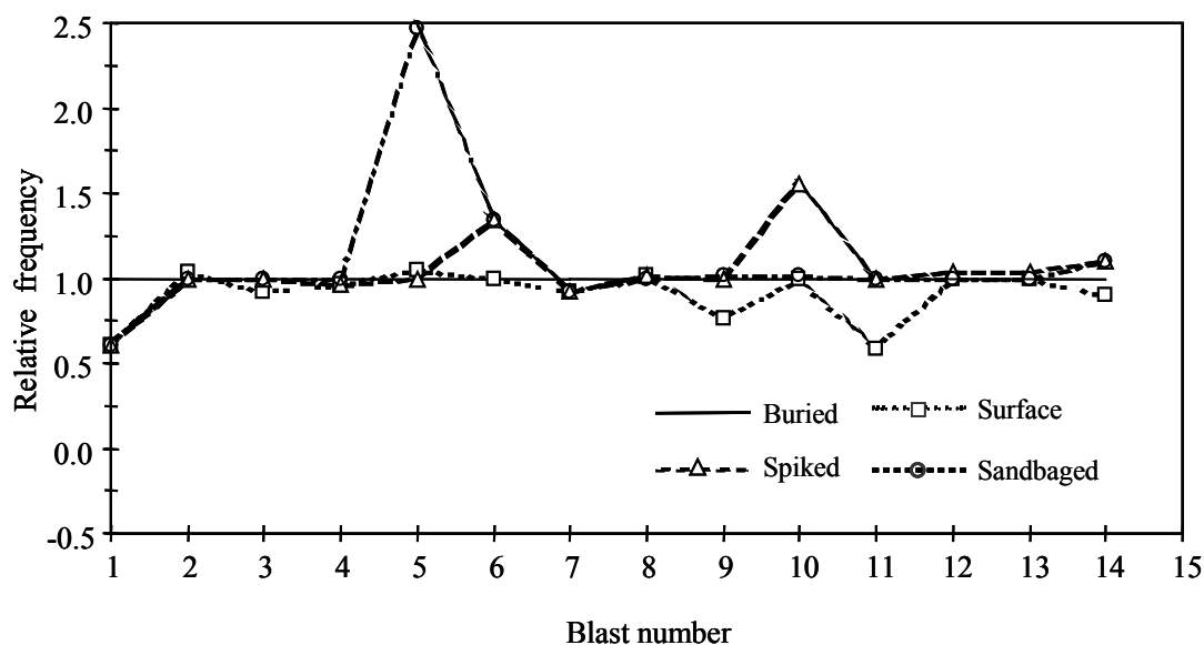
Fig. 4.4 Influence of transducer mounting methods on frequency of ground motions
